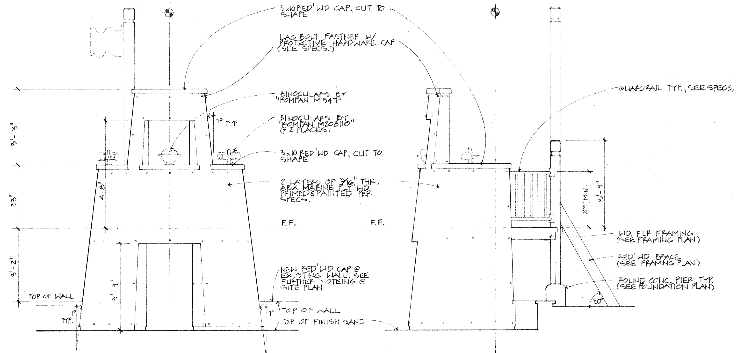
Elevation K
